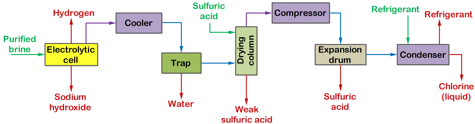
Figure: Manufacture of chlorine from salt by electrolysis
